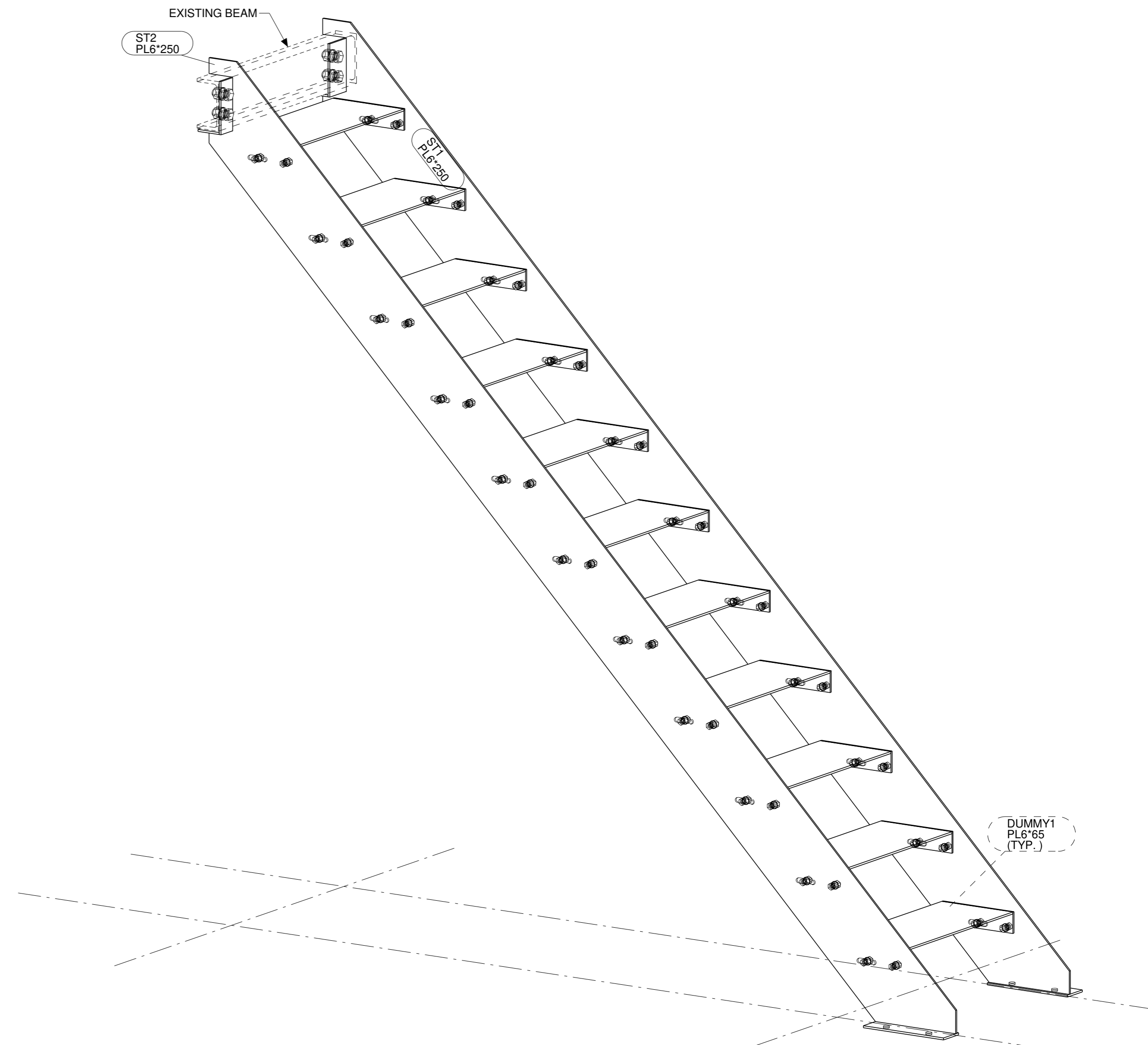
3D VIEW 1:10
