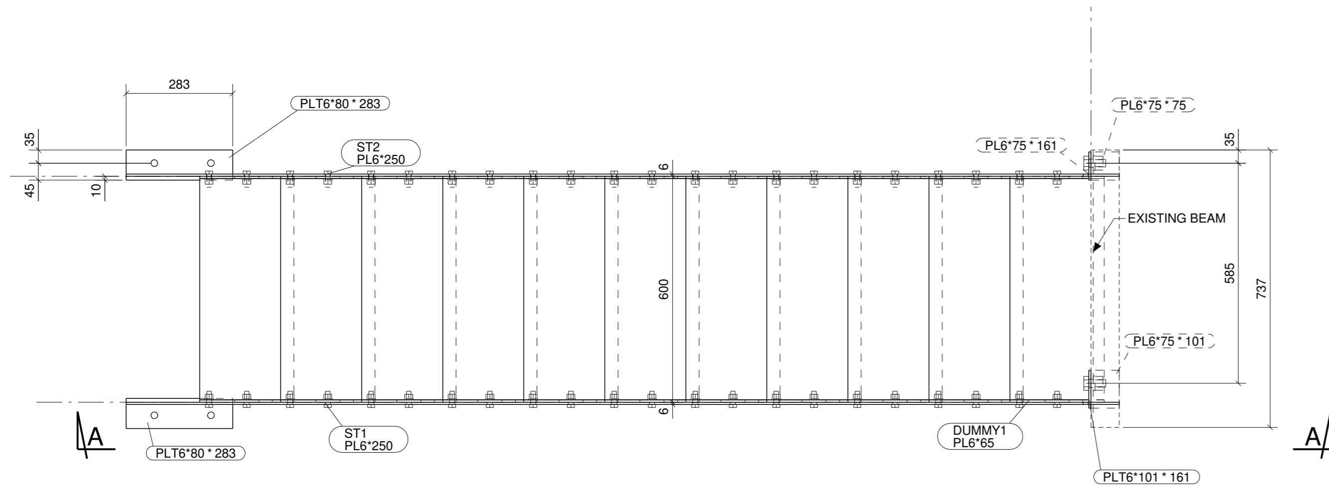
PLAN VIEW 1:10
